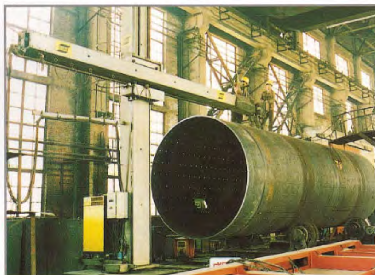
多功能自动焊机 Multi-functional automatic welding machine
