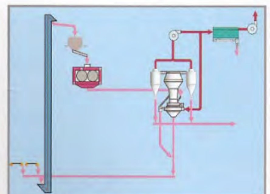
辊压机粉磨系统-终粉磨 Roller press finish grinding
