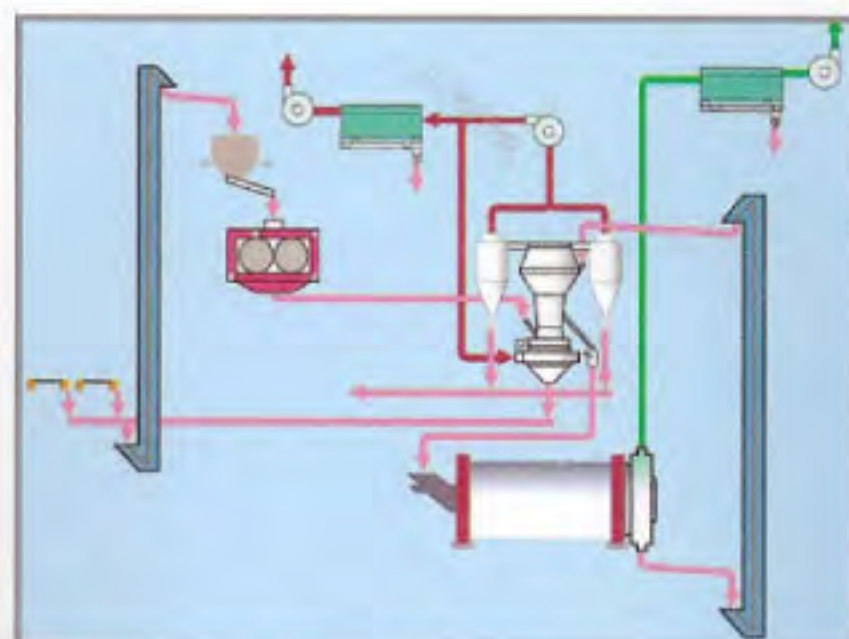
辊压机粉磨系统-半终粉磨 Roller press semi-finish grinding
