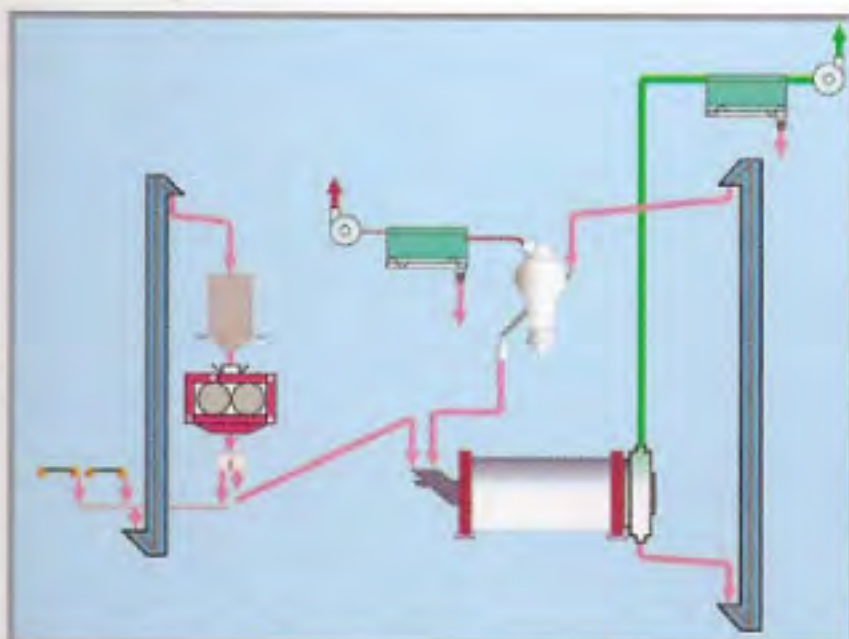
辊压机粉磨系统-预粉磨 Roller press pre-grinding
